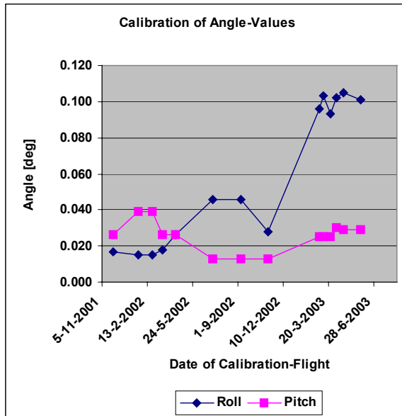
Figure 10: Results of pitch and roll angle calibration
