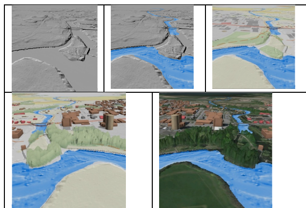
Figure 7 The 2.5D landscape model with buildings (blow) of Lantmateriet
