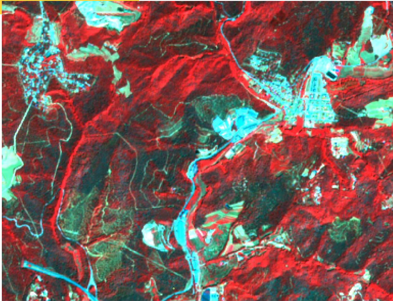
Sentinel-2 2017
