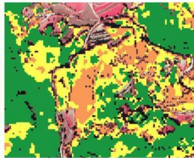
3 classes
